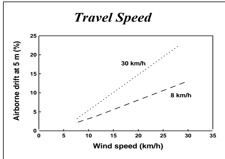
Effect of travel speed on spray drift. 30 km/h travel speed conducted using XR11002 tips applying 30 L/ha. 8 km/h travel speed done using XR8001 tips applying 50 L/ha.
