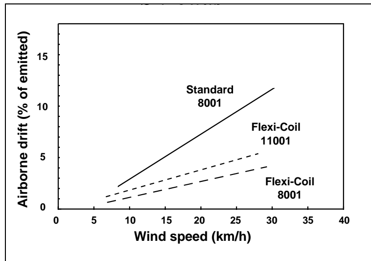
Reduction of drift with shrouds. Application volume was 50 L/ha.
