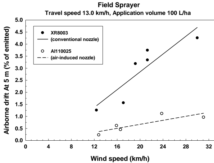
Effect of droplet size on off-target spray drift. Boom height was 60 cm.
